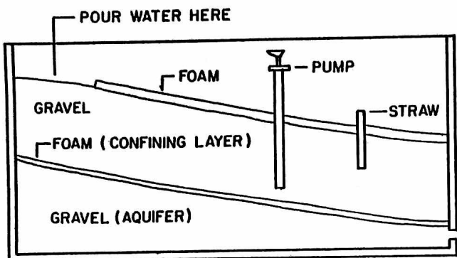
Fig. 1: BASIC GROUNDWATER MODEL
