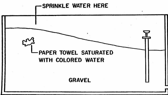
Fig. 3: LANDFILL / ABANDONED WASTE SITE MODEL
