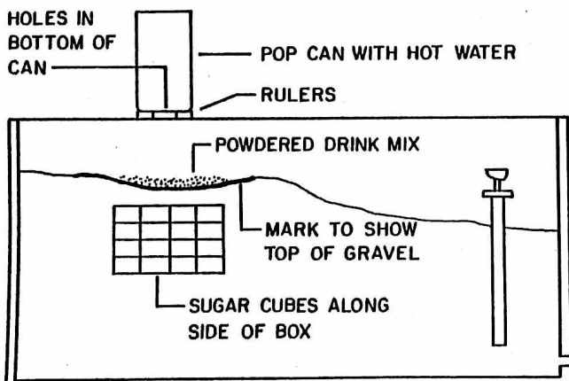
Fig. 7: SINKHOLE MODEL
