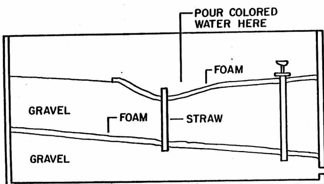
Fig. 5: AG-DRAINAGE WELL MODEL
